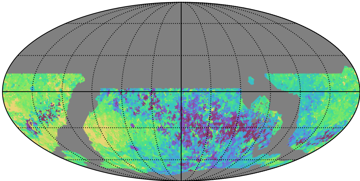
noroll_mjdp0_v3.4_10yrs WFD all bands: Max Inter-Night Gap
