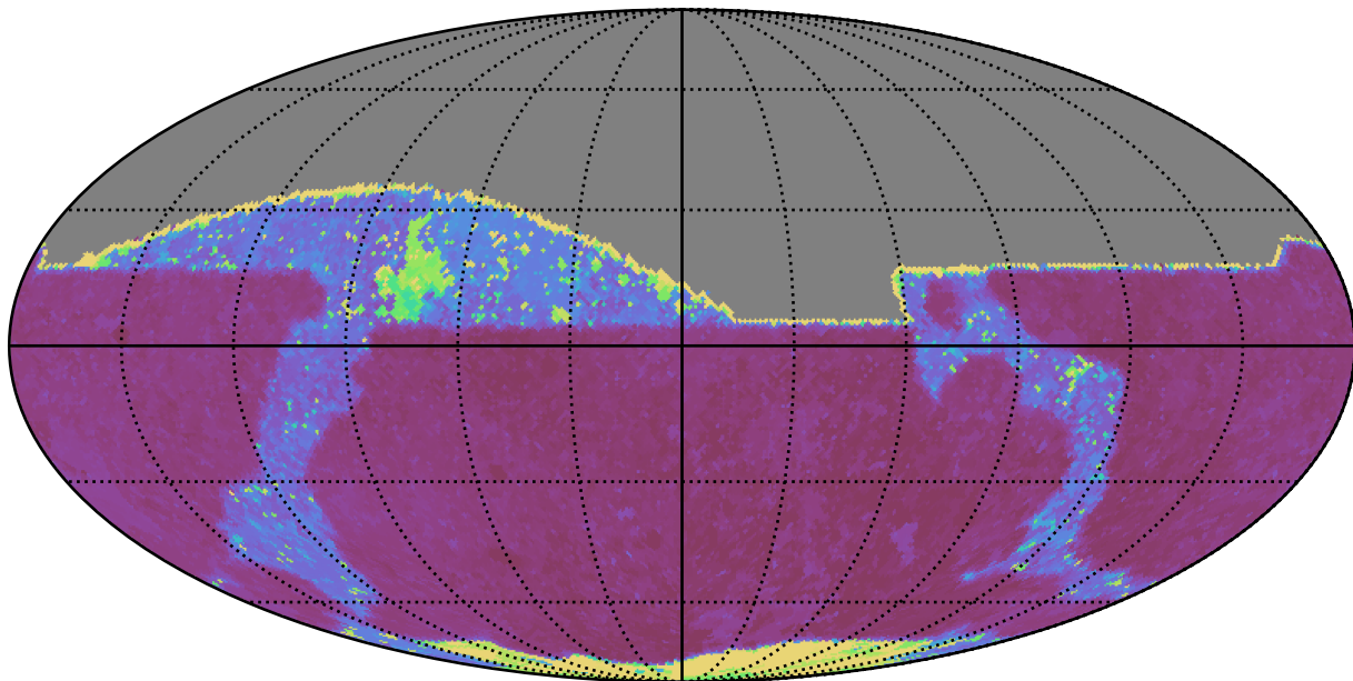
noroll_mjdp0_v3.4_10yrs All sky z band: Max Inter-Night Gap
