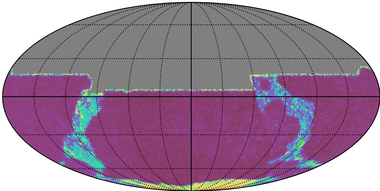
noroll_mjdp0_v3.4_10yrs All sky y band: Max Inter-Night Gap
