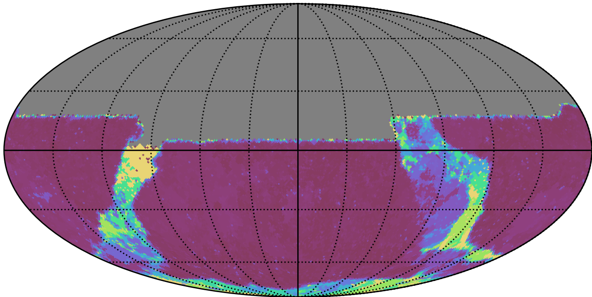
noroll_mjdp0_v3.4_10yrs All sky u band: Max Inter-Night Gap
