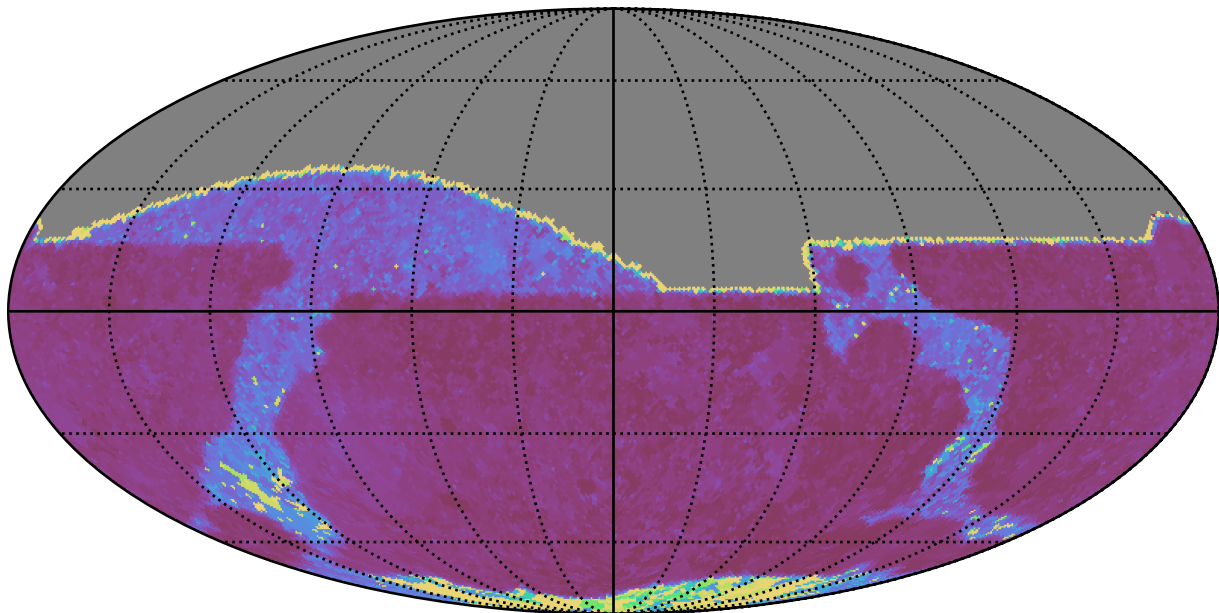
noroll_mjdp0_v3.4_10yrs All sky i band: Max Inter-Night Gap
