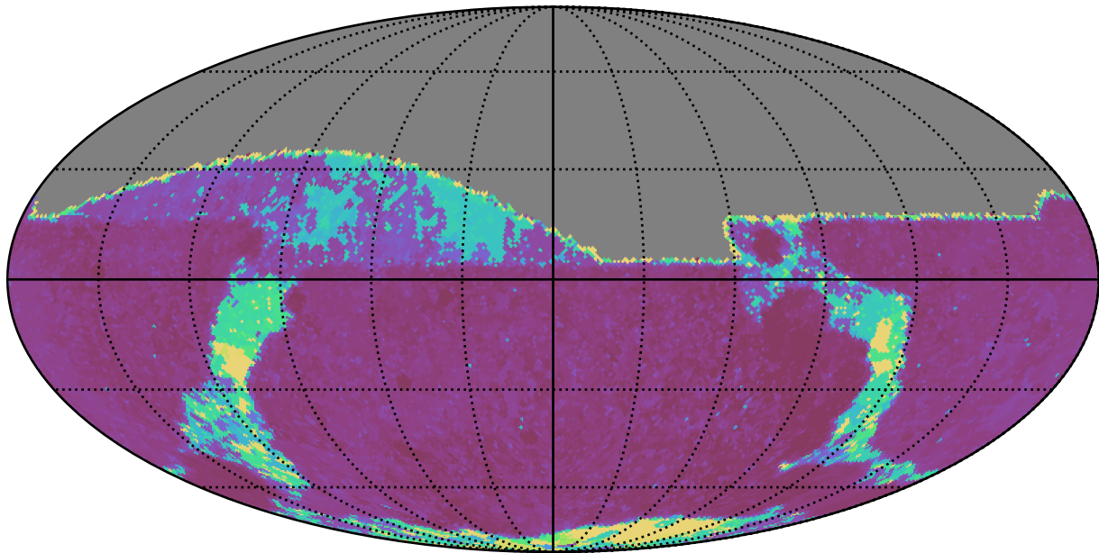
noroll_mjdp0_v3.4_10yrs All sky g band: Max Inter-Night Gap
