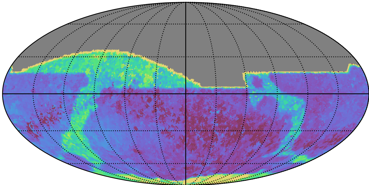
noroll_mjdp0_v3.4_10yrs All sky all bands: Max Inter-Night Gap
