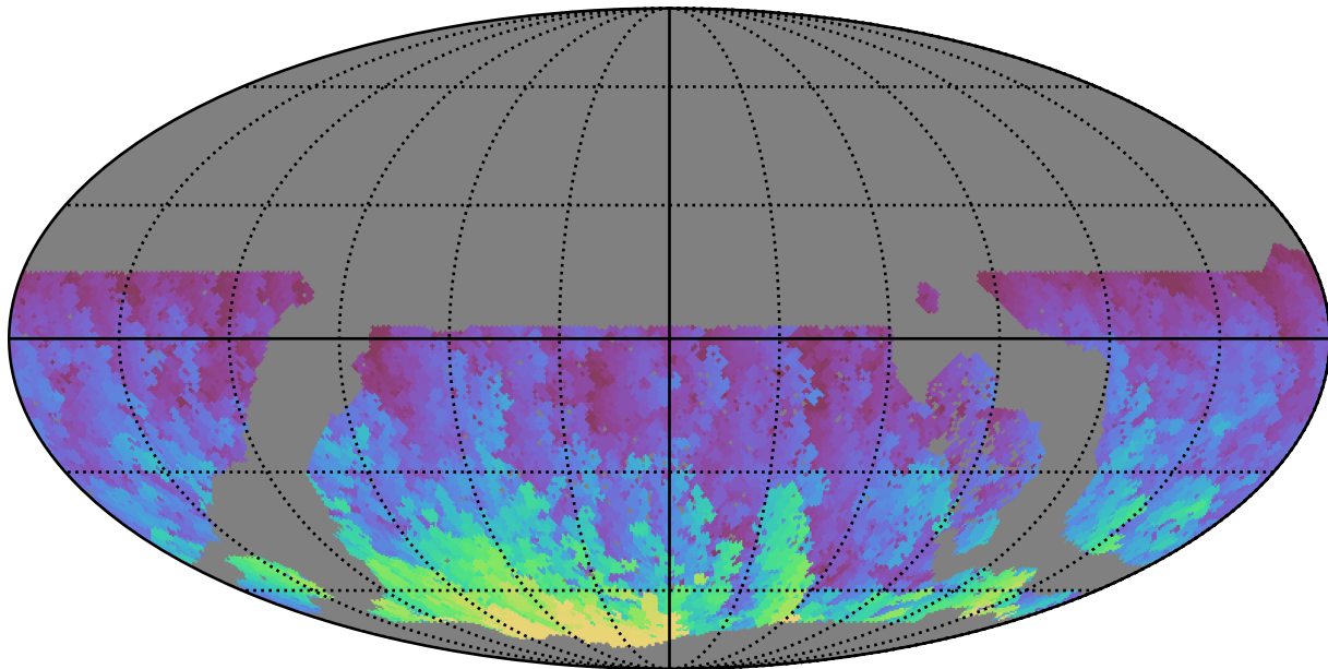
noroll_mjdp0_v3.4_10yrs WFD y band: Max HA
