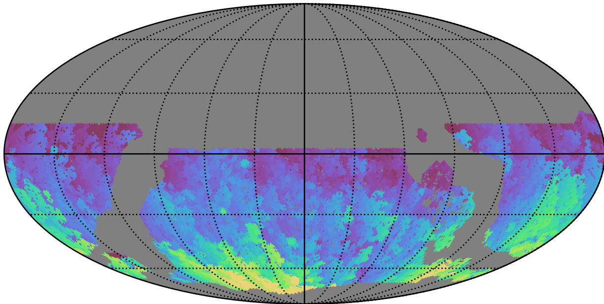
noroll_mjdp0_v3.4_10yrs WFD u band: Max HA
