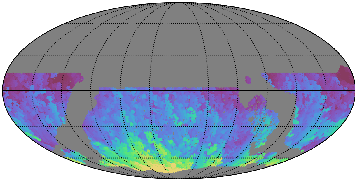
noroll_mjdp0_v3.4_10yrs WFD r band: Max HA
