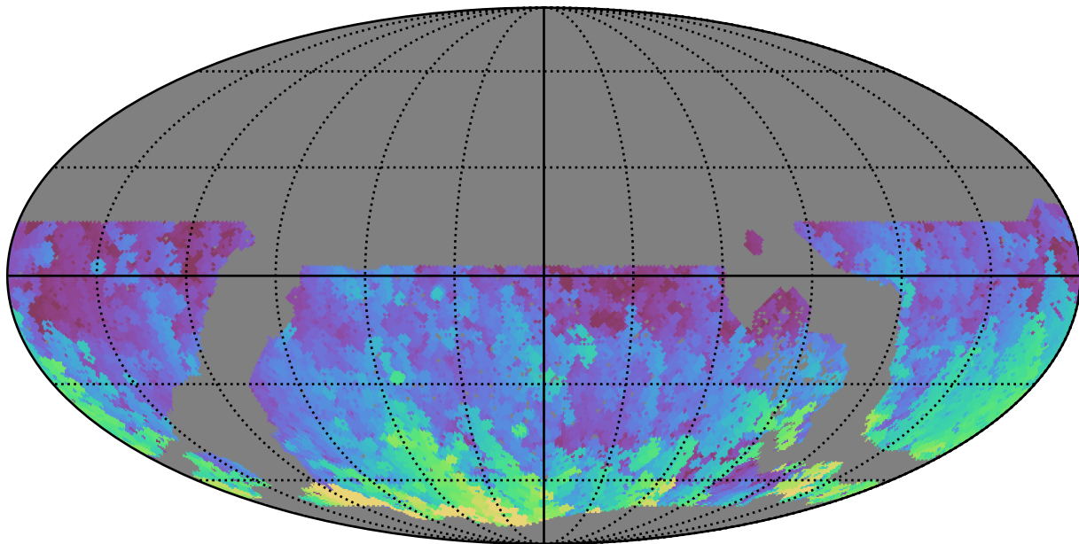
noroll_mjdp0_v3.4_10yrs WFD g band: Max HA
