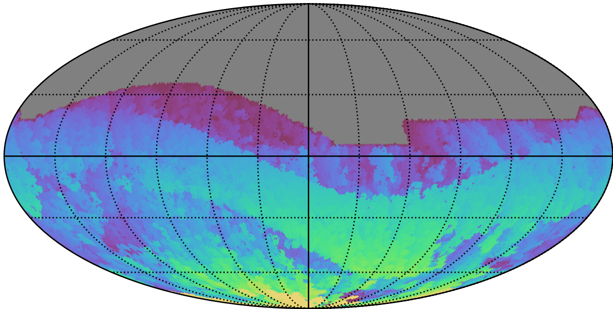
noroll_mjdp0_v3.4_10yrs All sky z band: Max HA
