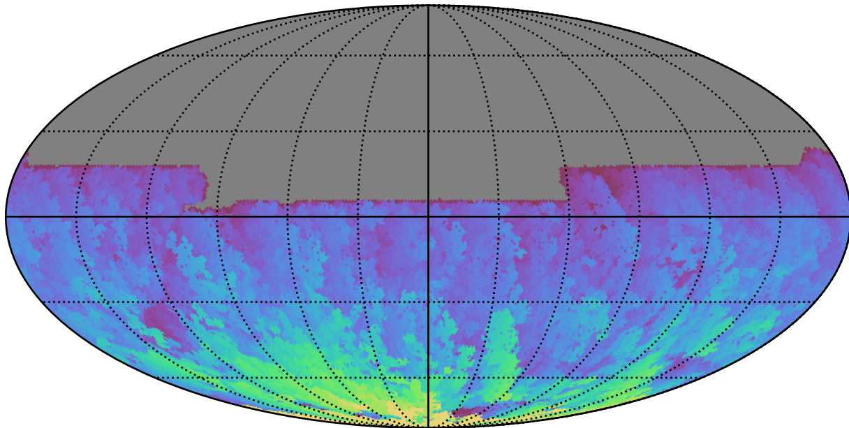
noroll_mjdp0_v3.4_10yrs All sky y band: Max HA
