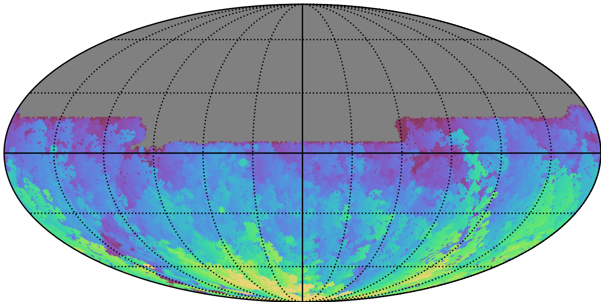
noroll_mjdp0_v3.4_10yrs All sky u band: Max HA
