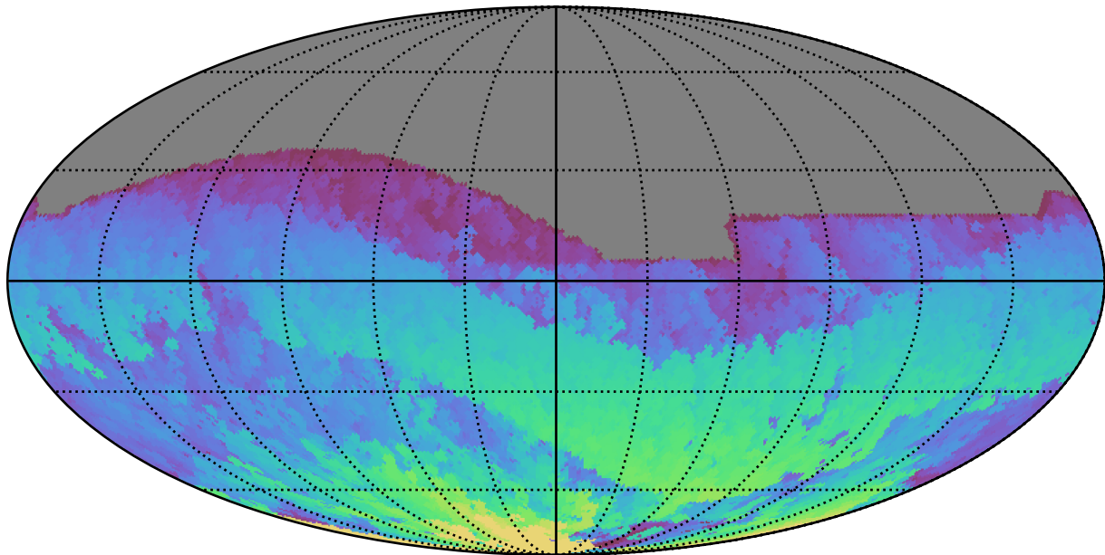
noroll_mjdp0_v3.4_10yrs All sky i band: Max HA
