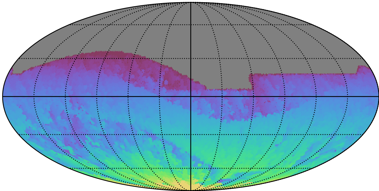
noroll_mjdp0_v3.4_10yrs All sky all bands: Max HA
