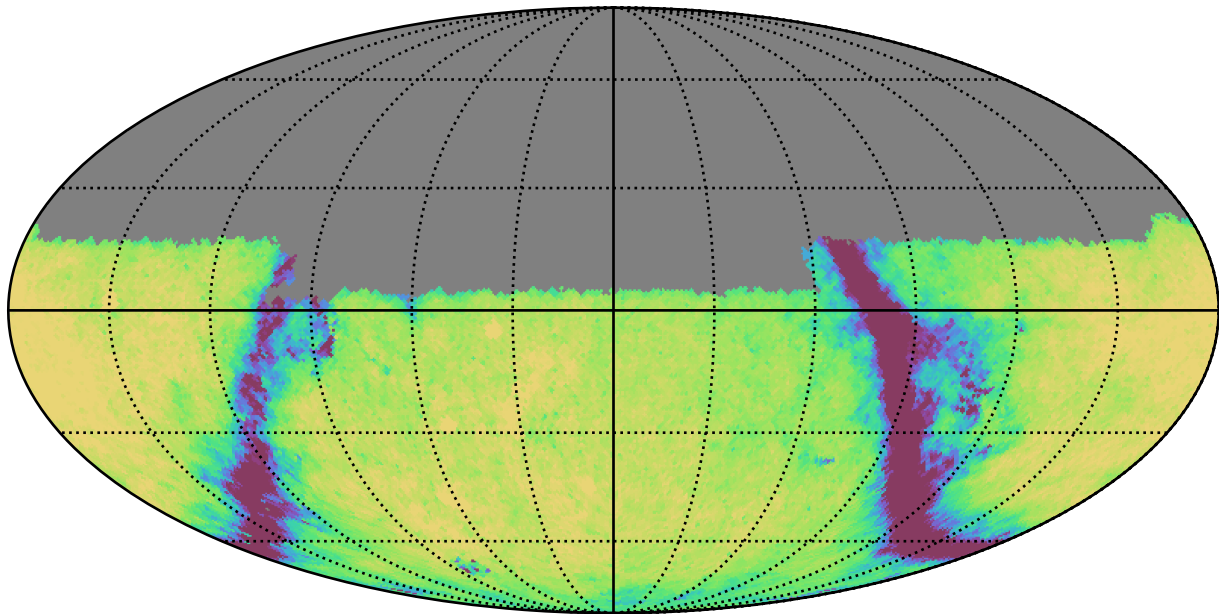
noroll_mjdp0_v3.4_10yrs Yr 1 u band: Exgal_CoaddM5
