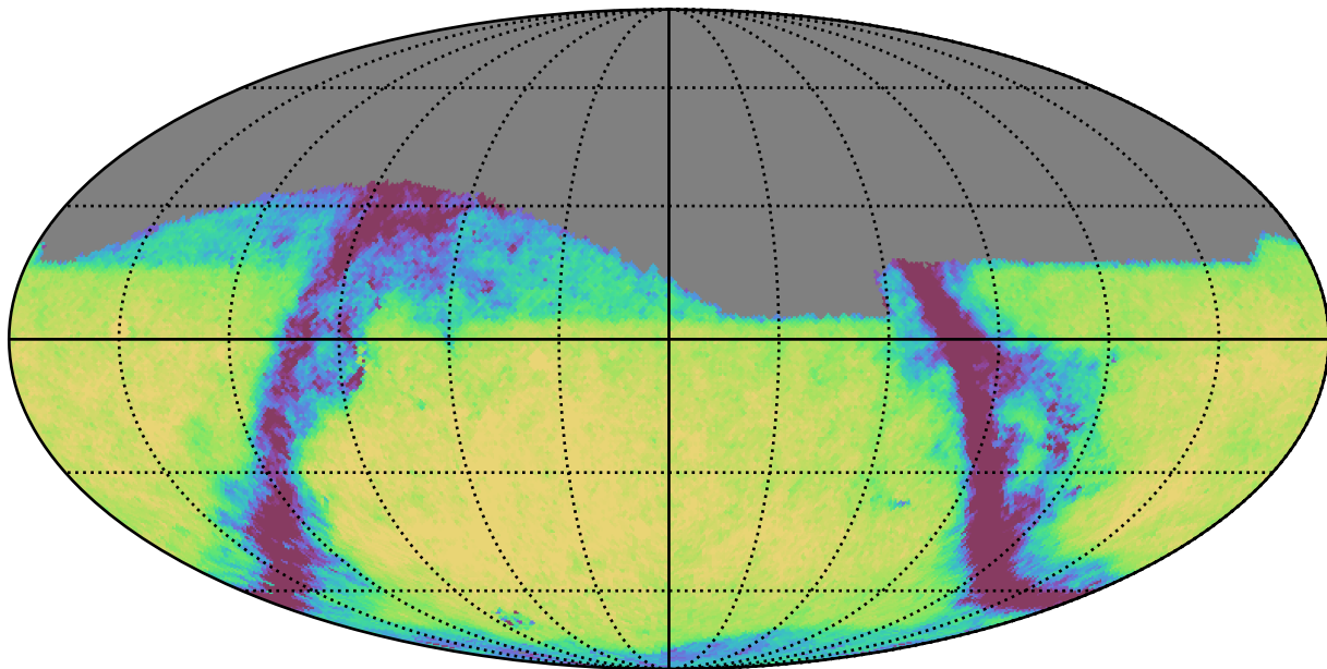
noroll_mjdp0_v3.4_10yrs Yr 1 r band: Exgal_CoaddM5
