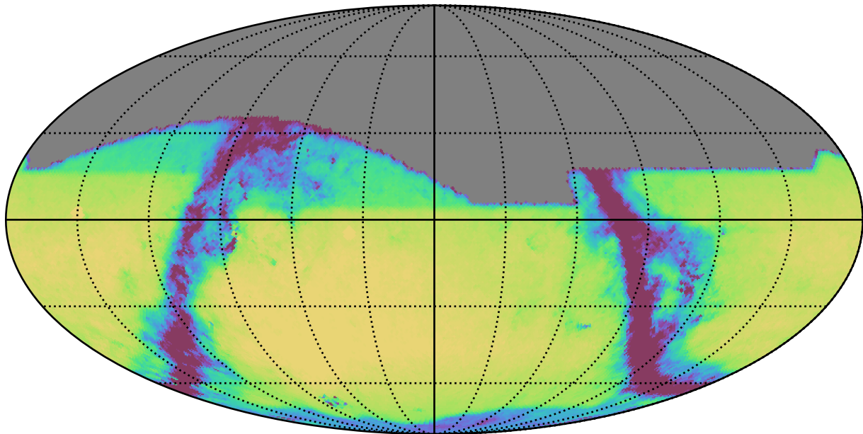
noroll_mjdp0_v3.4_10yrs All sky r band: Exgal_CoaddM5
