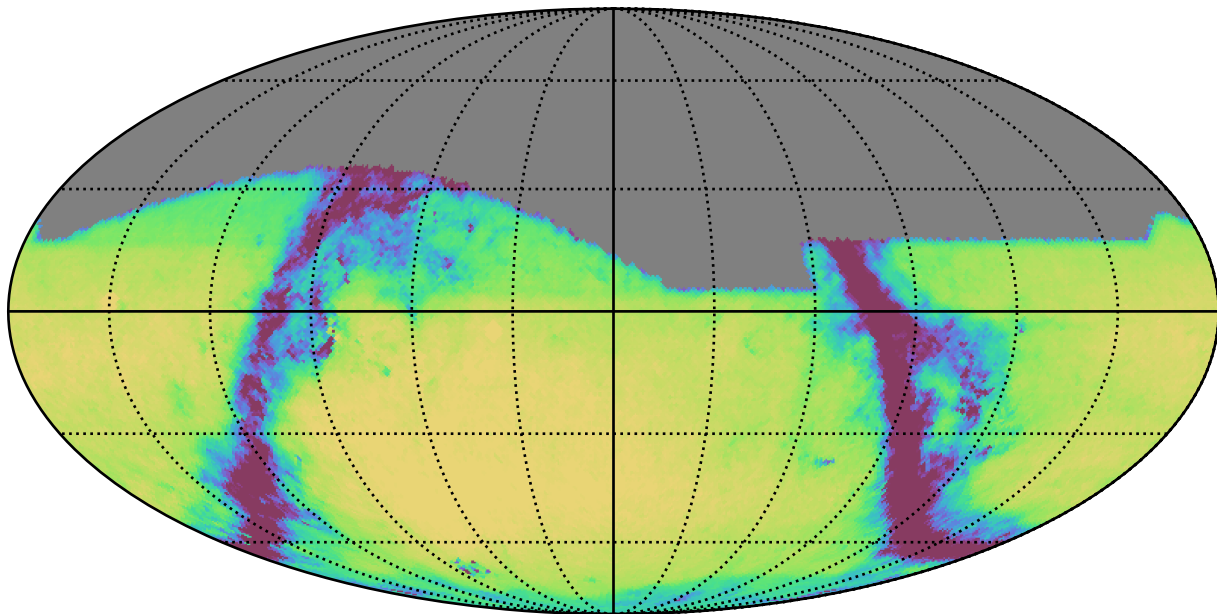
noroll_mjdp0_v3.4_10yrs All sky g band: Exgal_CoaddM5
