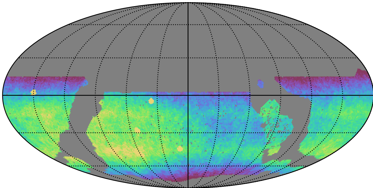
noroll_mjdp0_v3.4_10yrs WFD r band: CoaddM5
