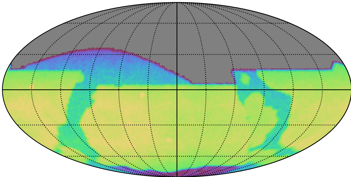
noroll_mjdp0_v3.4_10yrs All sky z band: CoaddM5
