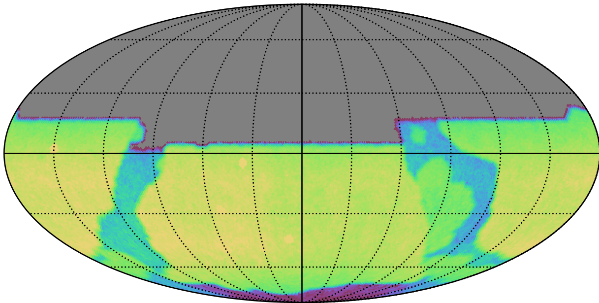
noroll_mjdp0_v3.4_10yrs All sky y band: CoaddM5
