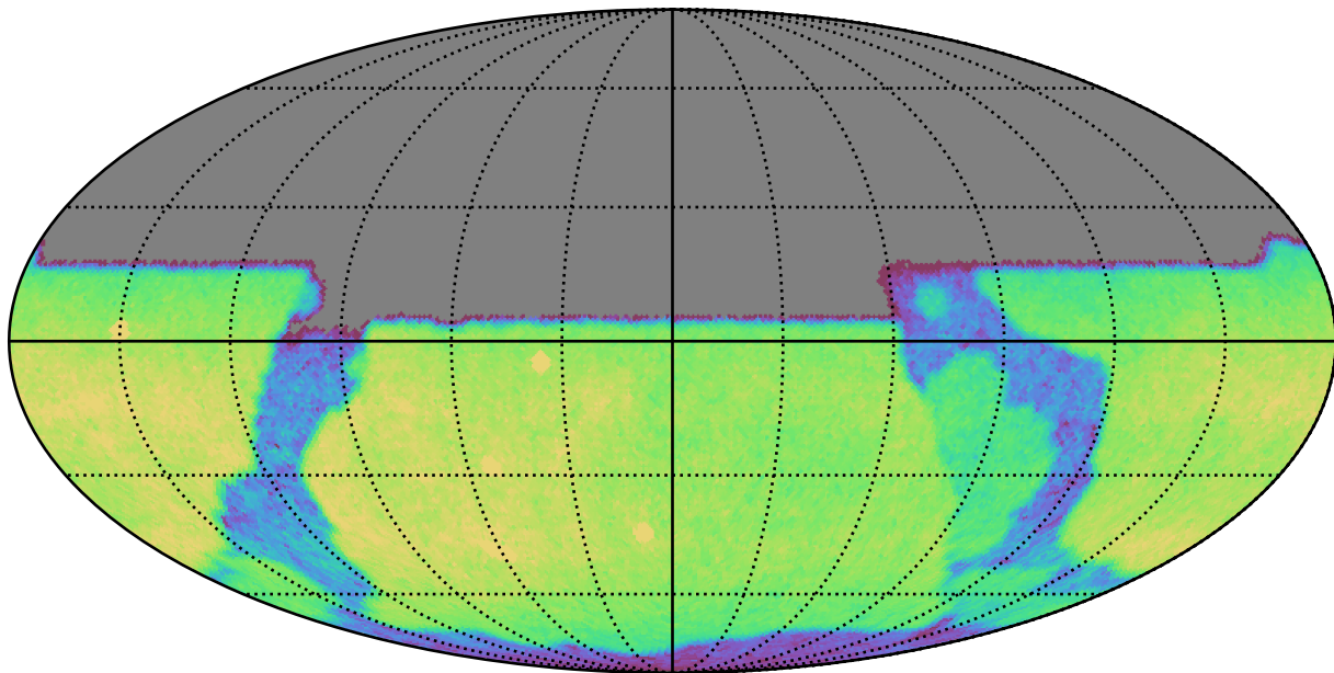
noroll_mjdp0_v3.4_10yrs All sky u band: CoaddM5
