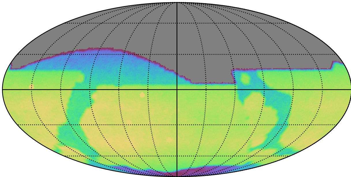
noroll_mjdp0_v3.4_10yrs All sky r band: CoaddM5
