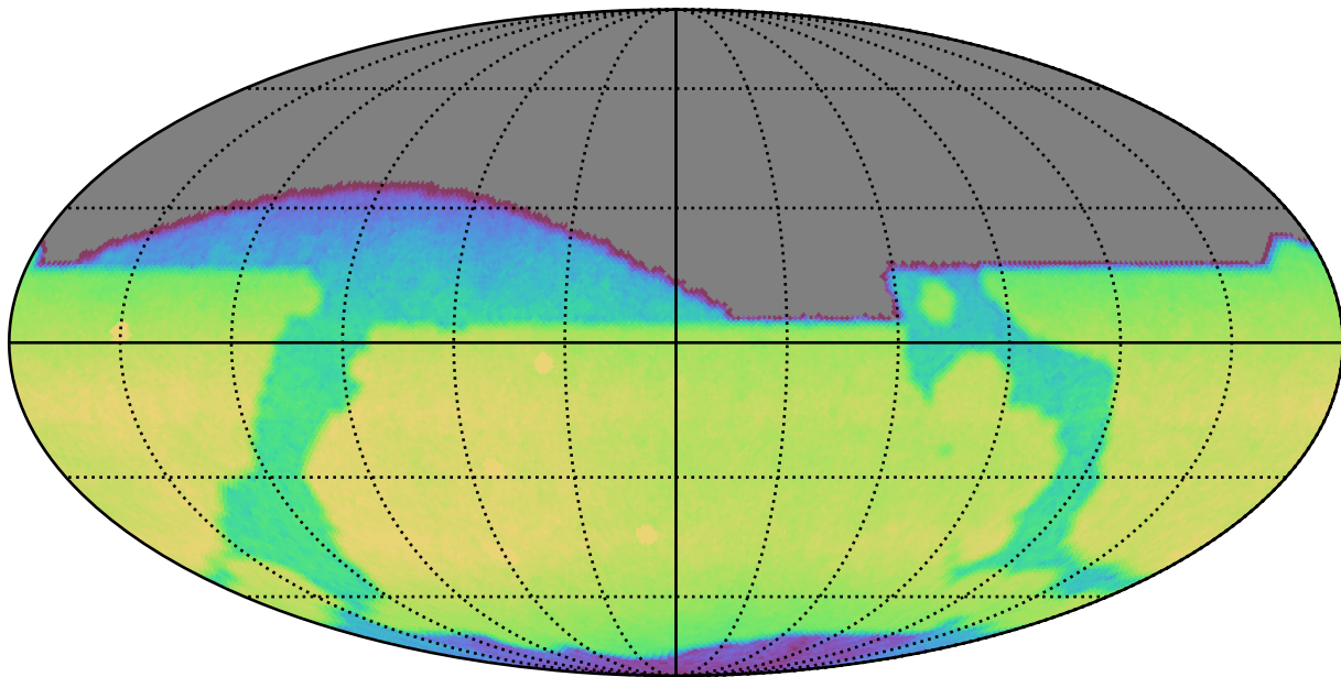
noroll_mjdp0_v3.4_10yrs All sky i band: CoaddM5
