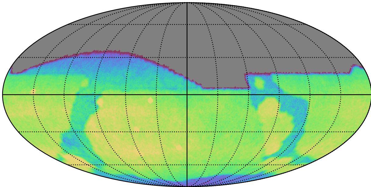
noroll_mjdp0_v3.4_10yrs All sky g band: CoaddM5
