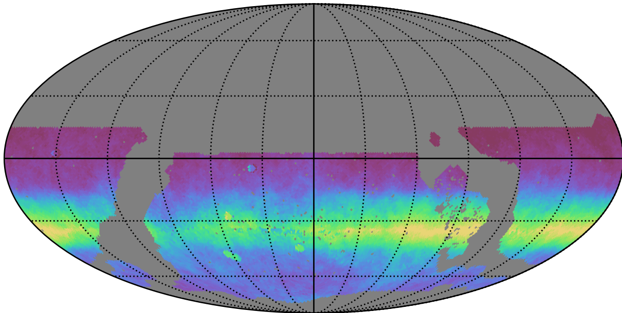
noroll_mjdp0_v3.4_10yrs WFD all bands: AngleRms rotSkyPos
