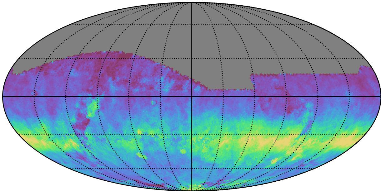
noroll_mjdp0_v3.4_10yrs All sky z band: AngleRms rotSkyPos
