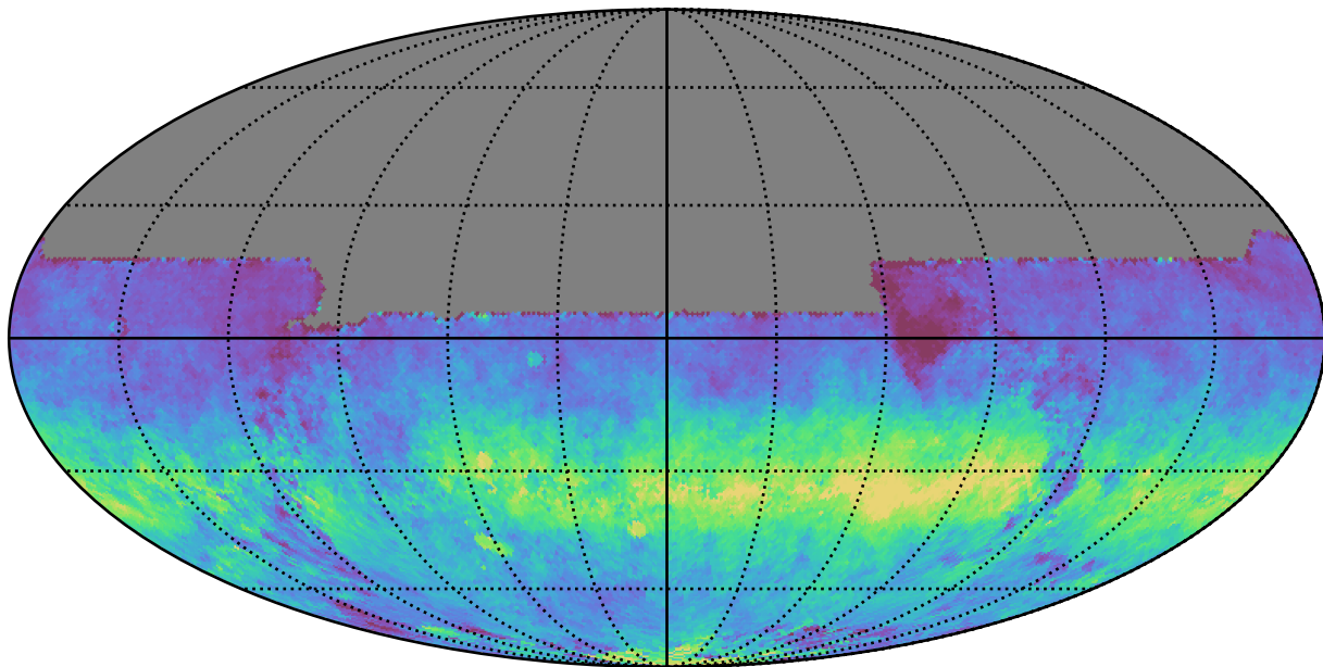
noroll_mjdp0_v3.4_10yrs All sky y band: AngleRms rotSkyPos
