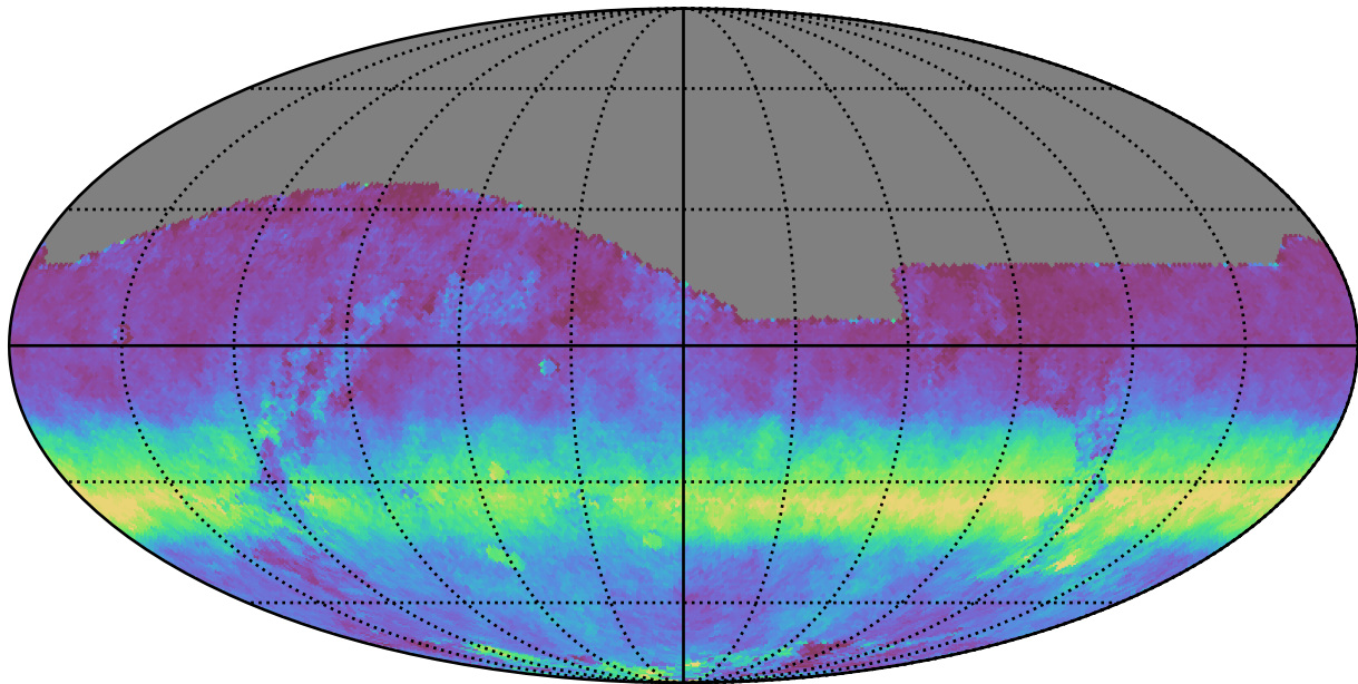
noroll_mjdp0_v3.4_10yrs All sky r band: AngleRms rotSkyPos
