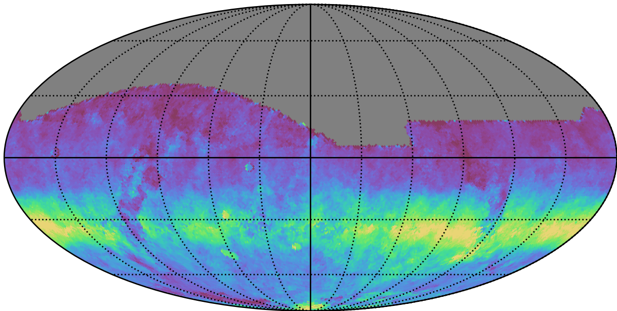
noroll_mjdp0_v3.4_10yrs All sky i band: AngleRms rotSkyPos
