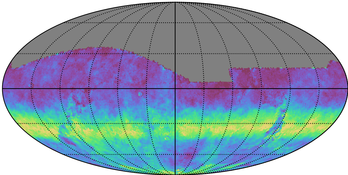
noroll_mjdp0_v3.4_10yrs All sky g band: AngleRms rotSkyPos
