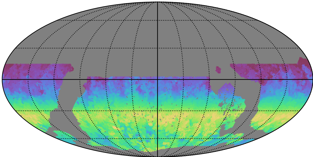
noroll_mjdp0_v3.4_10yrs WFD z band: AngleRange rotSkyPos
