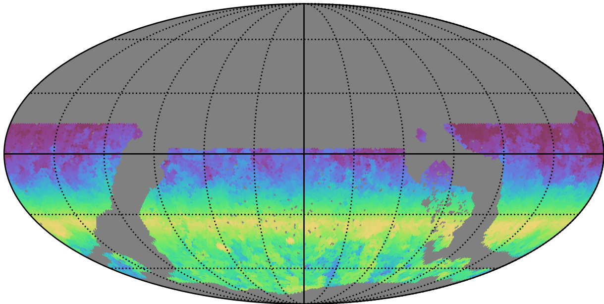
noroll_mjdp0_v3.4_10yrs WFD r band: AngleRange rotSkyPos
