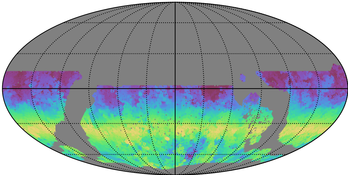
noroll_mjdp0_v3.4_10yrs WFD g band: AngleRange rotSkyPos
