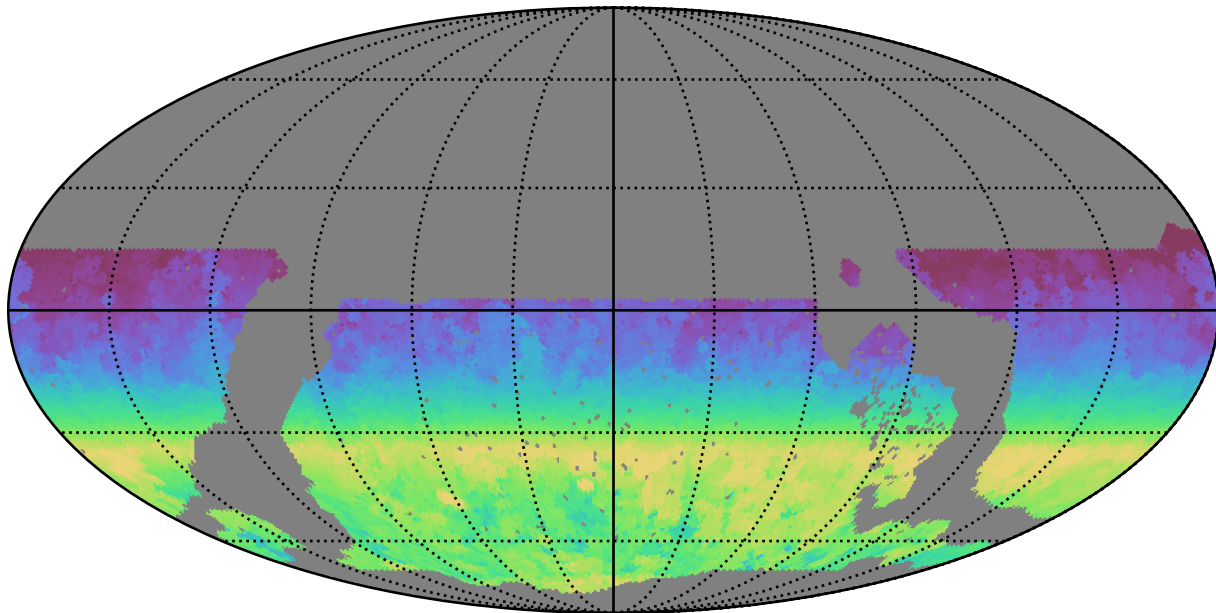
noroll_mjdp0_v3.4_10yrs WFD all bands: AngleRange rotSkyPos
