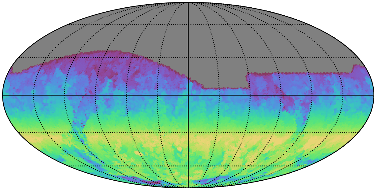
noroll_mjdp0_v3.4_10yrs All sky i band: AngleRange rotSkyPos
