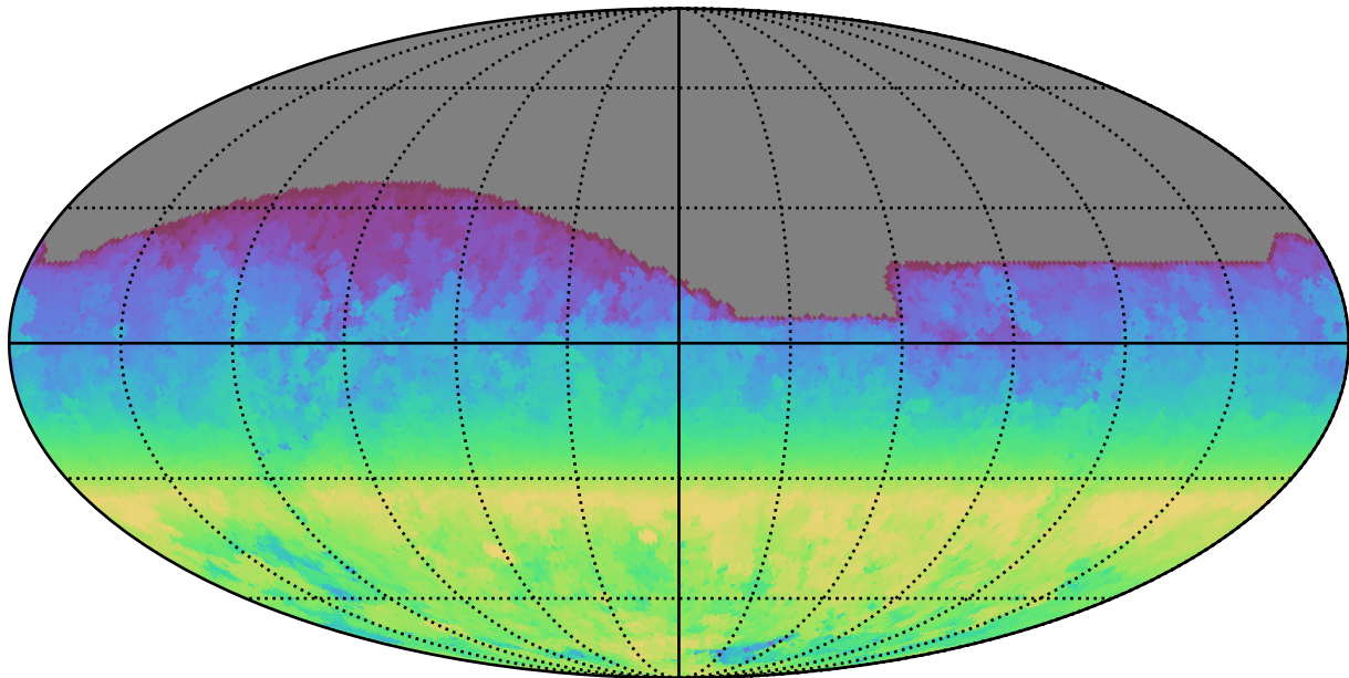
noroll_mjdp0_v3.4_10yrs All sky all bands: AngleRange rotSkyPos
