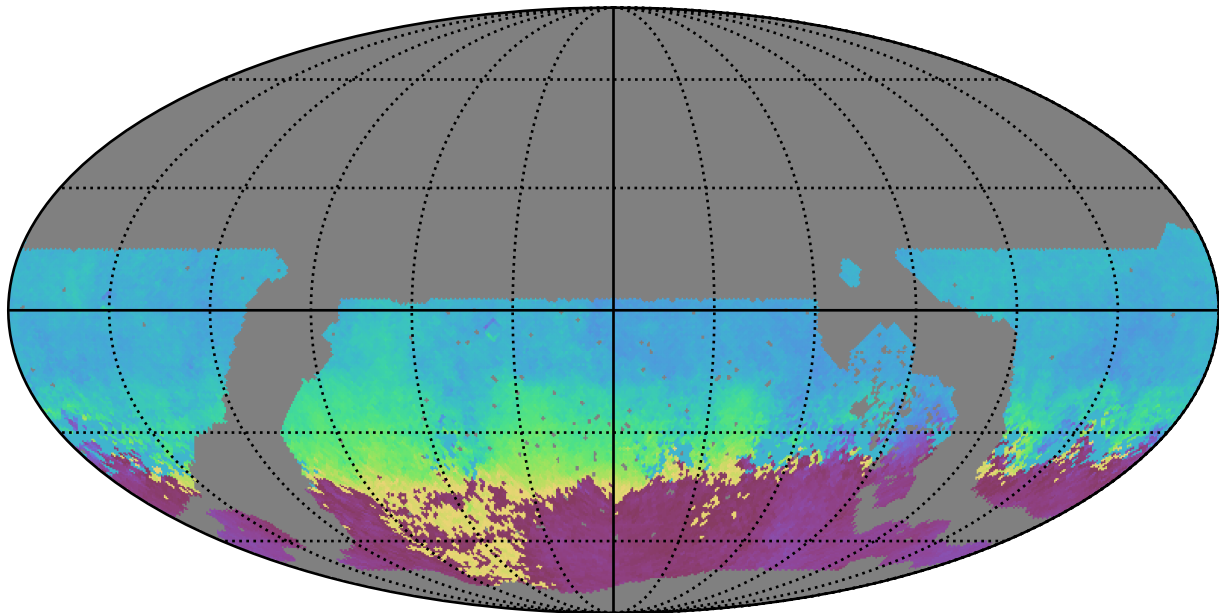
noroll_mjdp0_v3.4_10yrs WFD g band: AngleMean rotSkyPos
