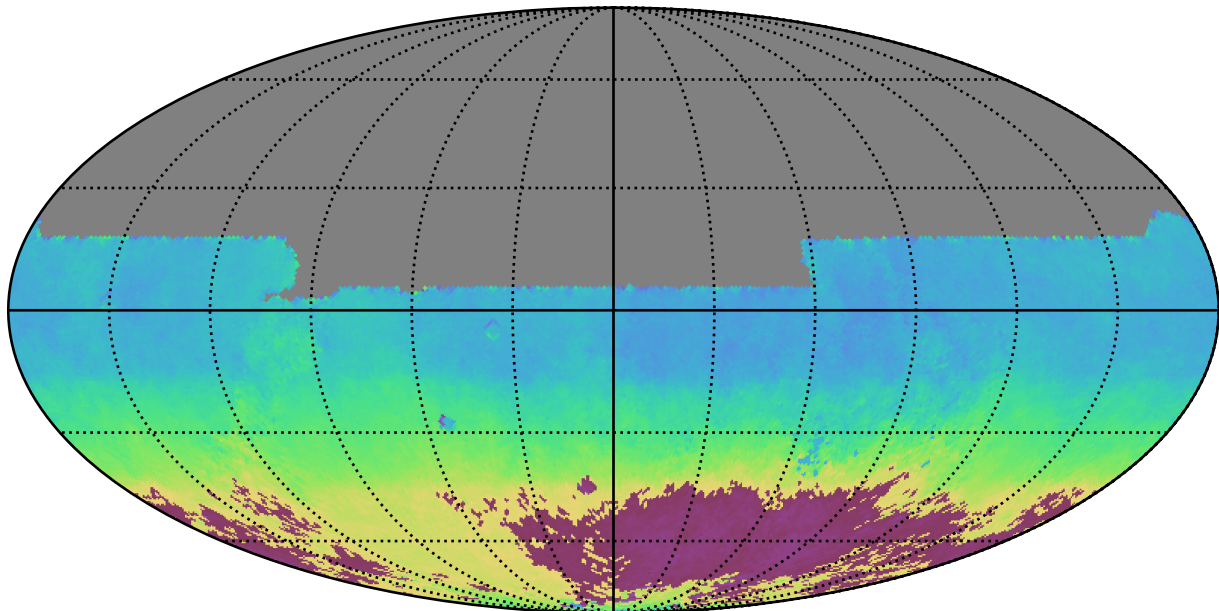
noroll_mjdp0_v3.4_10yrs All sky y band: AngleMean rotSkyPos
