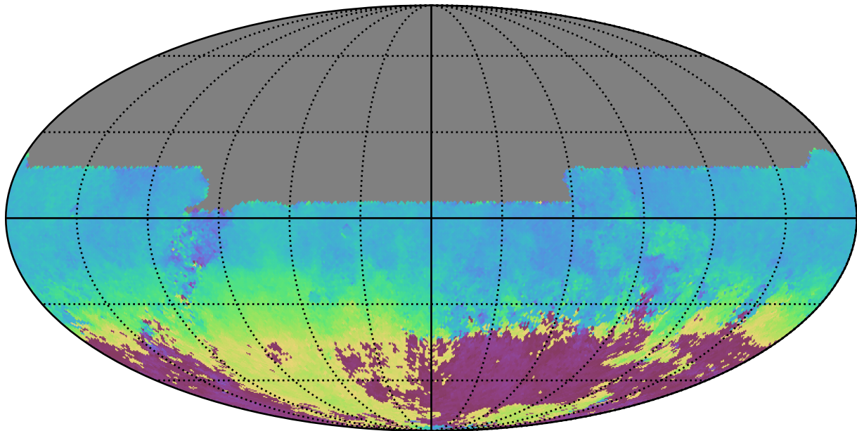
noroll_mjdp0_v3.4_10yrs All sky u band: AngleMean rotSkyPos
