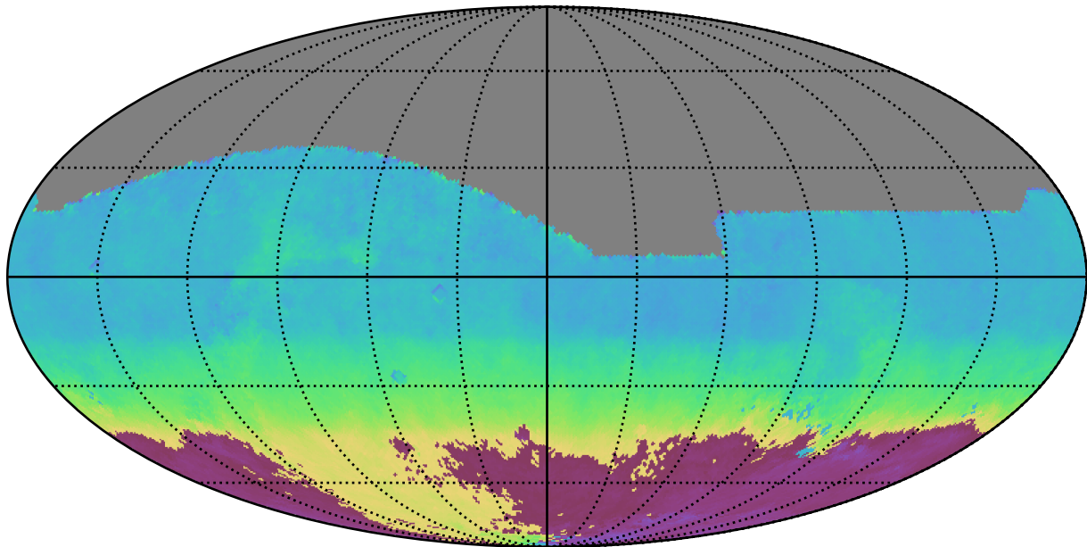
noroll_mjdp0_v3.4_10yrs All sky i band: AngleMean rotSkyPos
