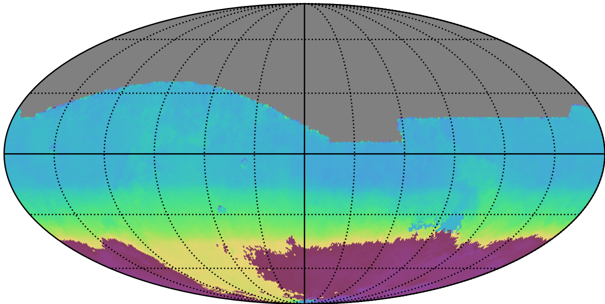
noroll_mjdp0_v3.4_10yrs All sky all bands: AngleMean rotSkyPos
