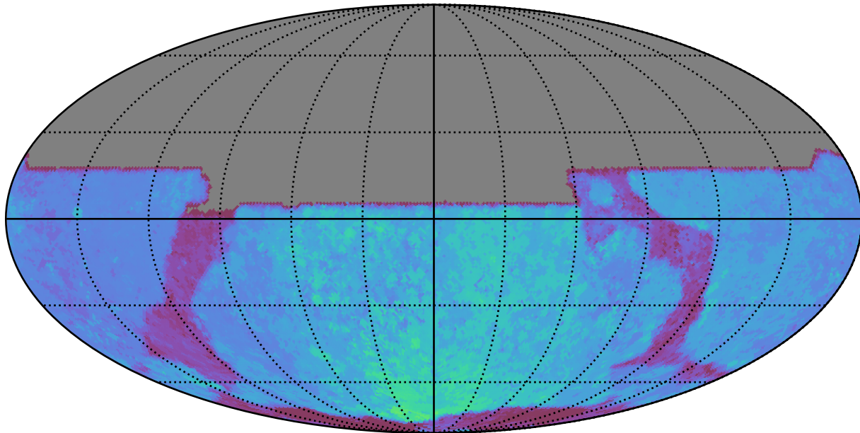
noroll_mjdp0_v3.4_10yrs All sky y band: 80thPercentile Season Length
