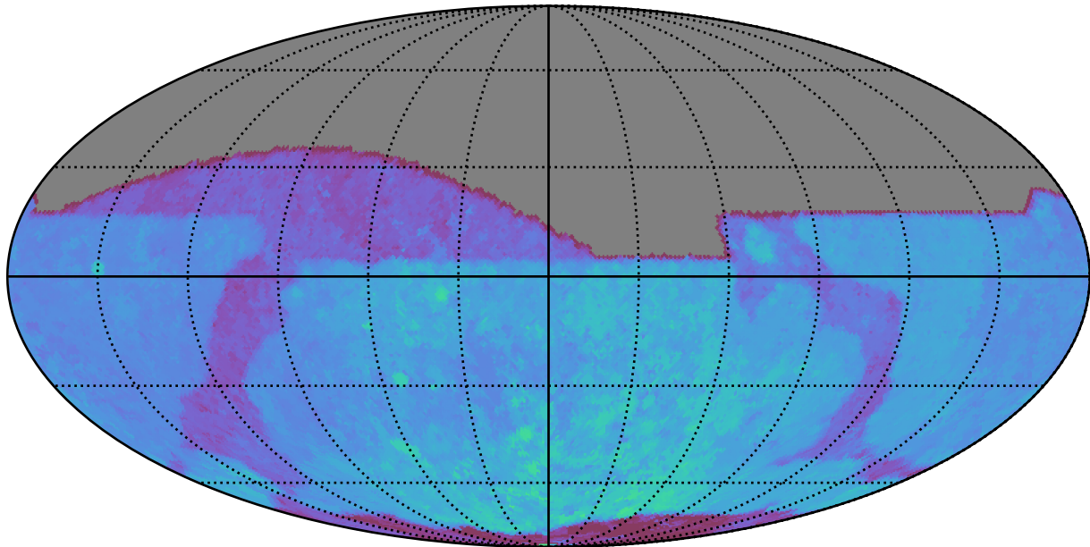
noroll_mjdp0_v3.4_10yrs All sky r band: 80thPercentile Season Length
