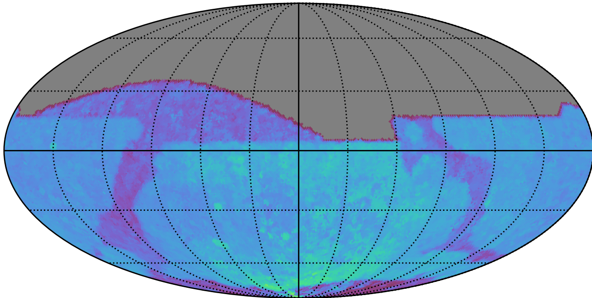
noroll_mjdp0_v3.4_10yrs All sky i band: 80thPercentile Season Length
