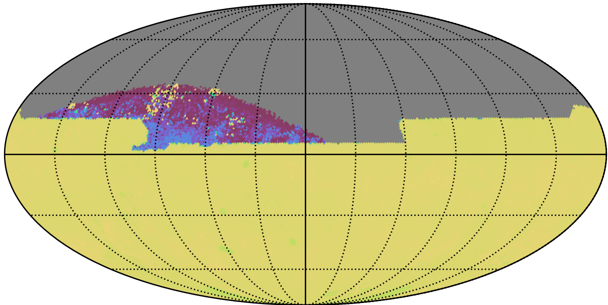
noroll_mjdp0_v3.4_10yrs All sky zy bands: 75th Percentile Intranight Timespan
