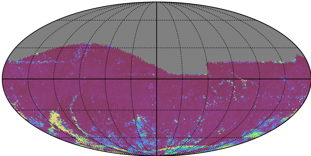
noroll_mjdp0_v3.4_10yrs All sky z band: 75th Percentile Intranight Timespan
