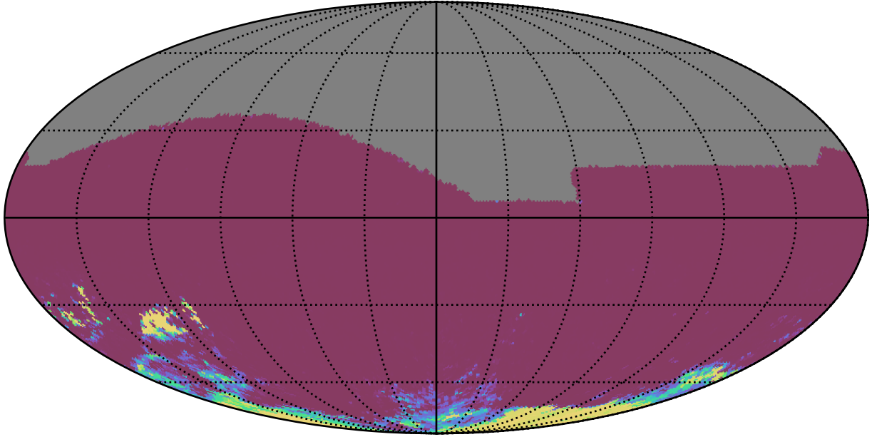
noroll_mjdp0_v3.4_10yrs All sky ri bands: 75th Percentile Intranight Timespan
